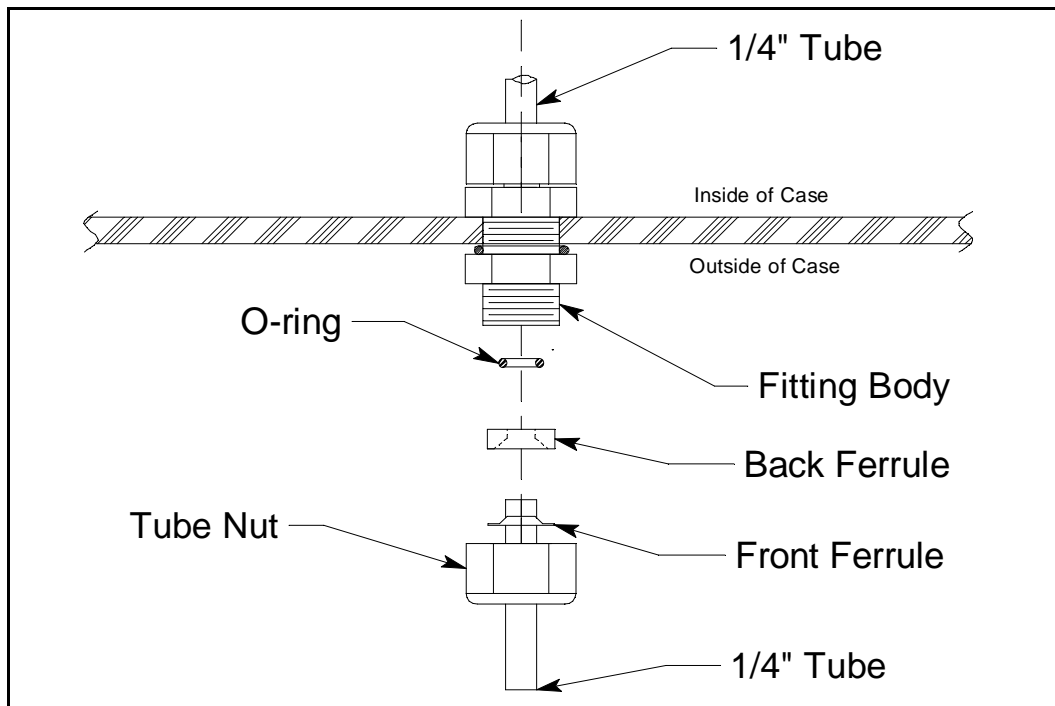
Figure 6: Inlet Fitting with Tubing Stub
