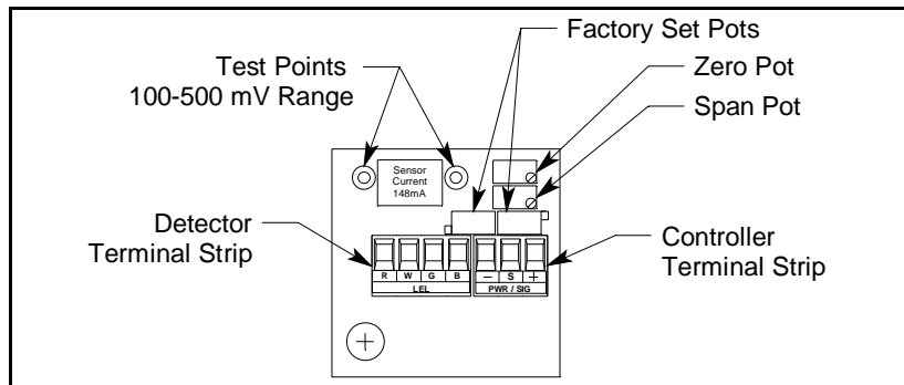
Figure 3: Amplifier Component Location
