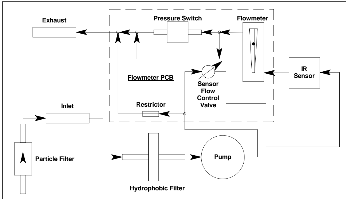
Figure 2: Sample-Draw Detector Flow Diagram
