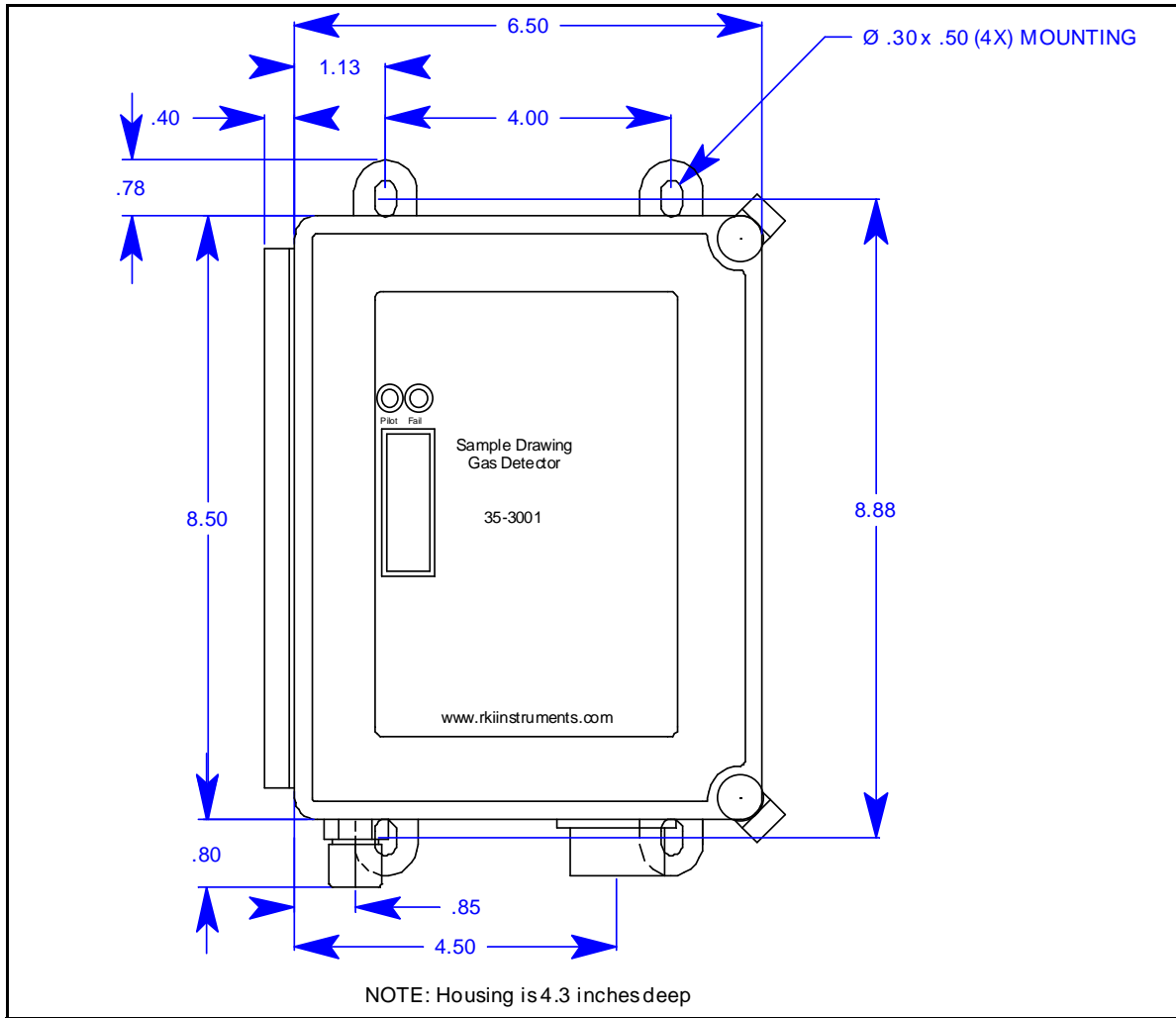
Figure 4: Outline and Mounting Dimensions
