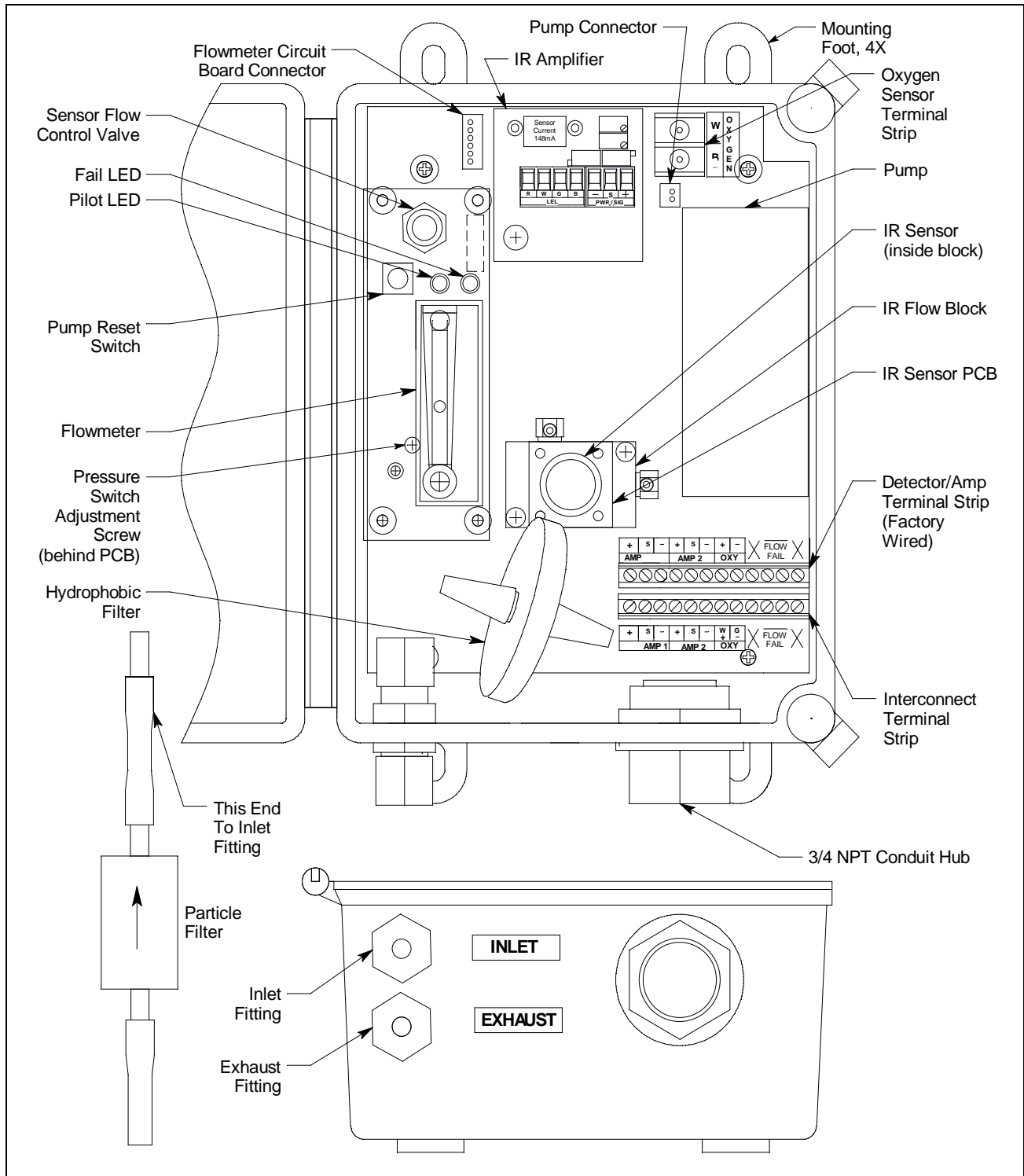
Figure 1: Sample-Draw Detector Component Location
