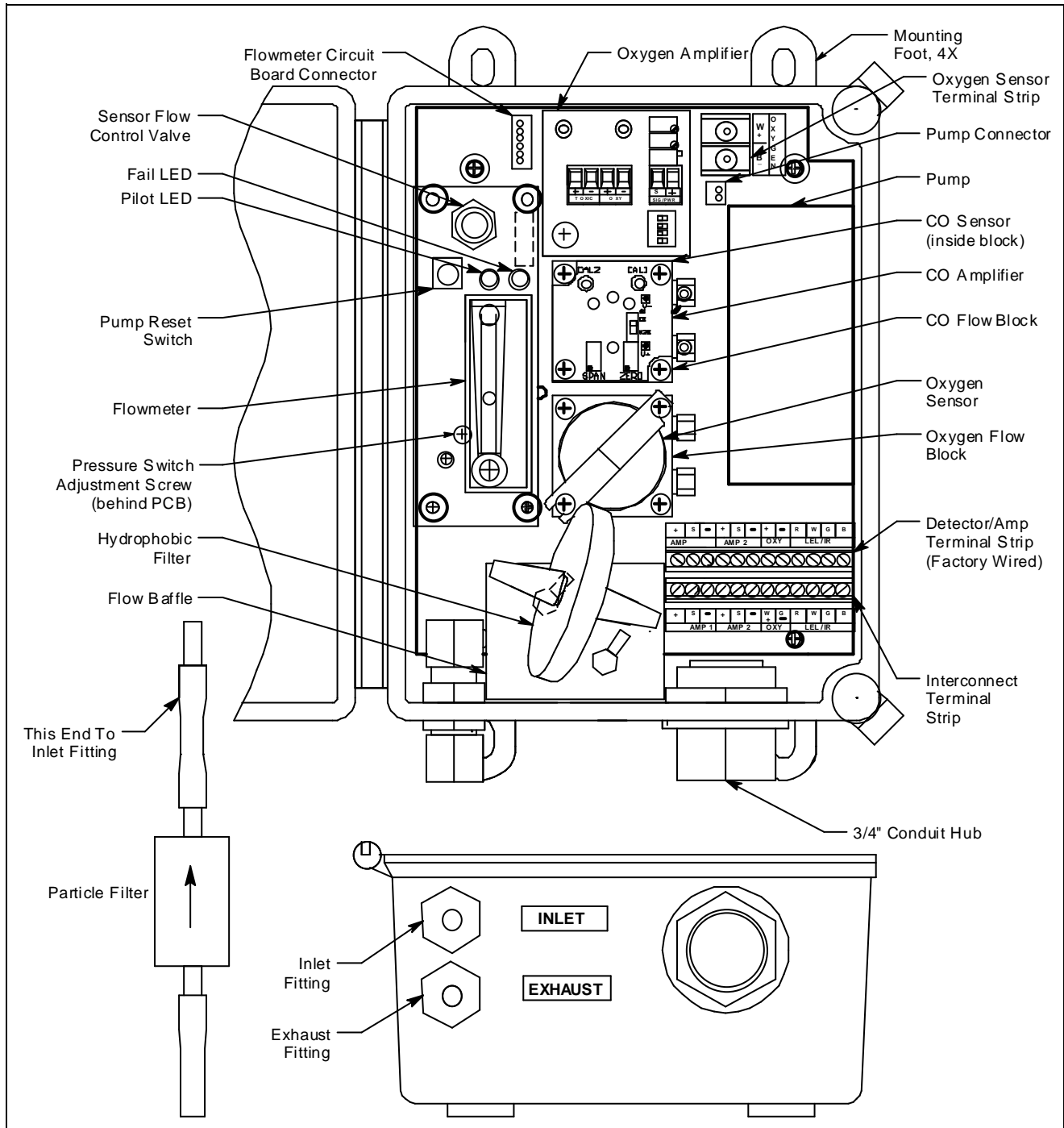
Figure 1: Component Location
