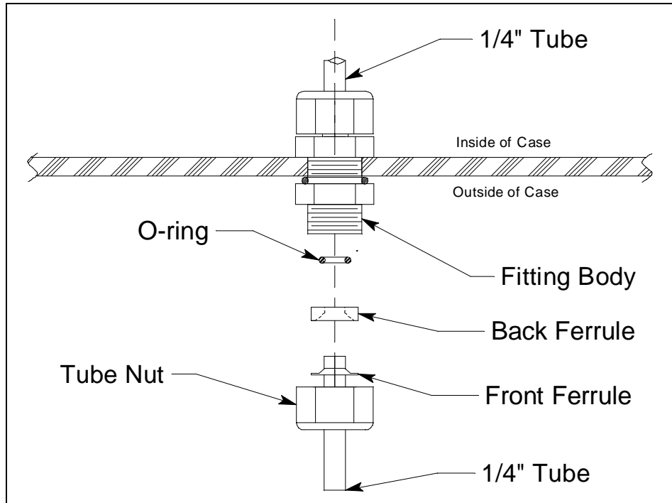
Figure 7: Inlet Fitting with Tubing Stub
