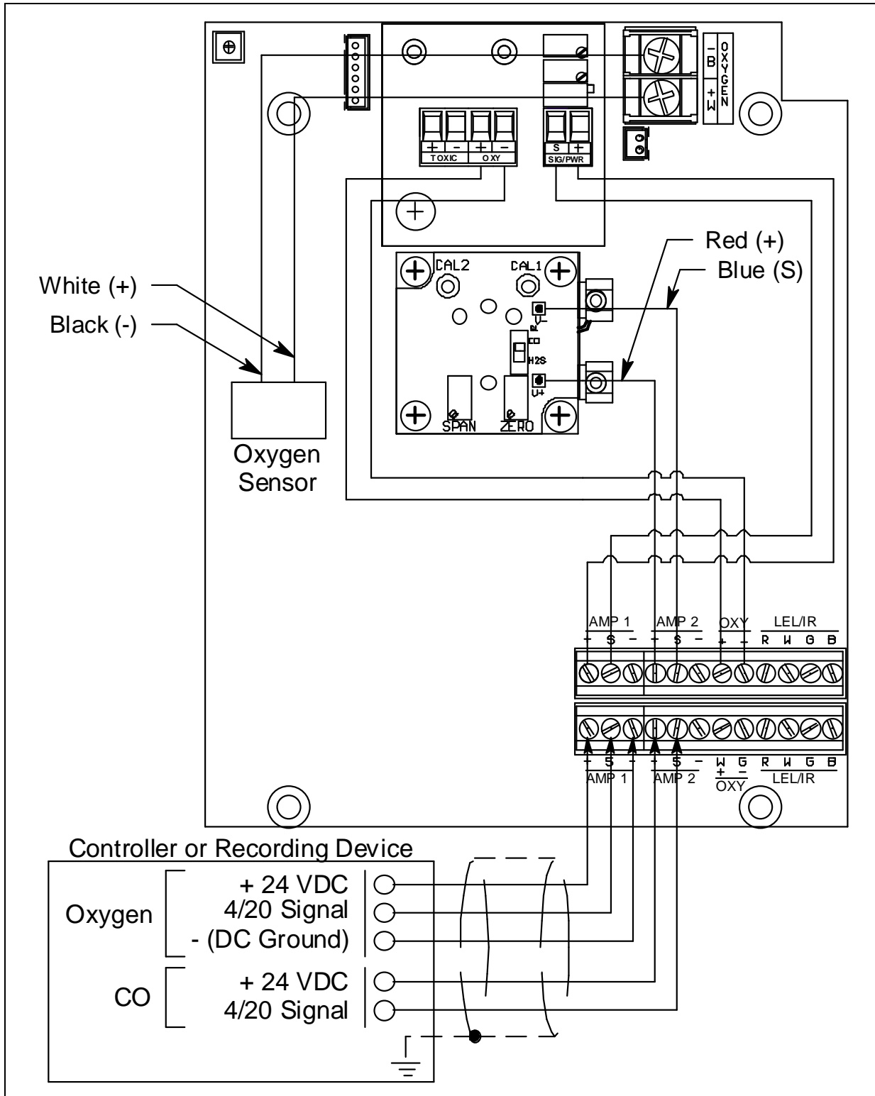
Figure 6: Wiring the Sample-Draw Detector to a Controller
