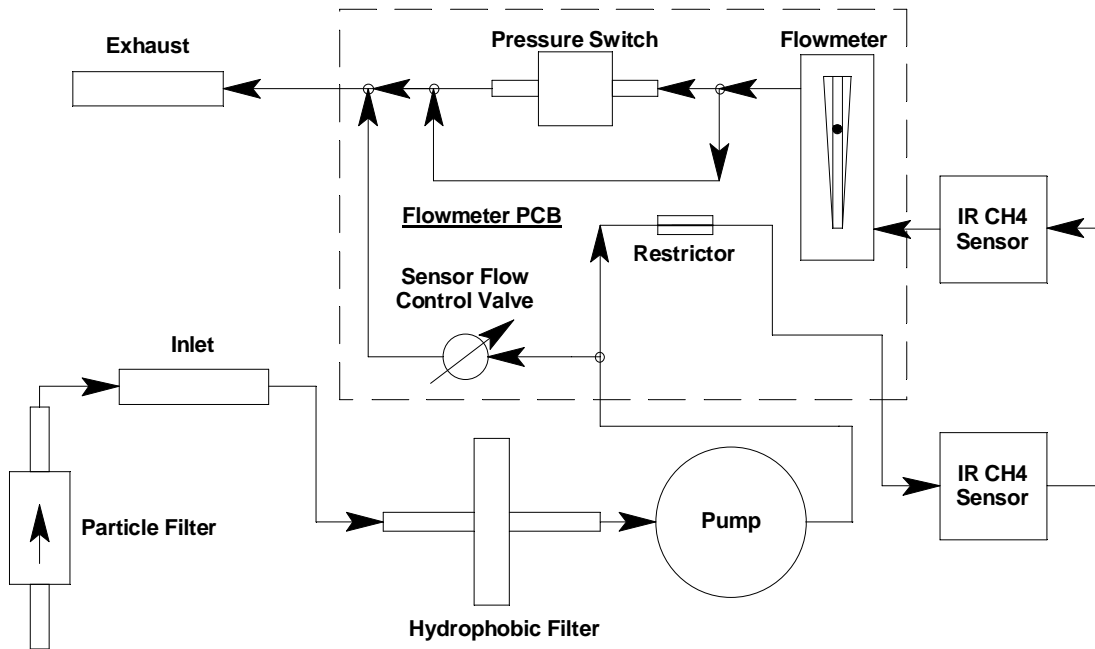
Figure 2: Methane Sample-Draw Detector Flow Diagram
