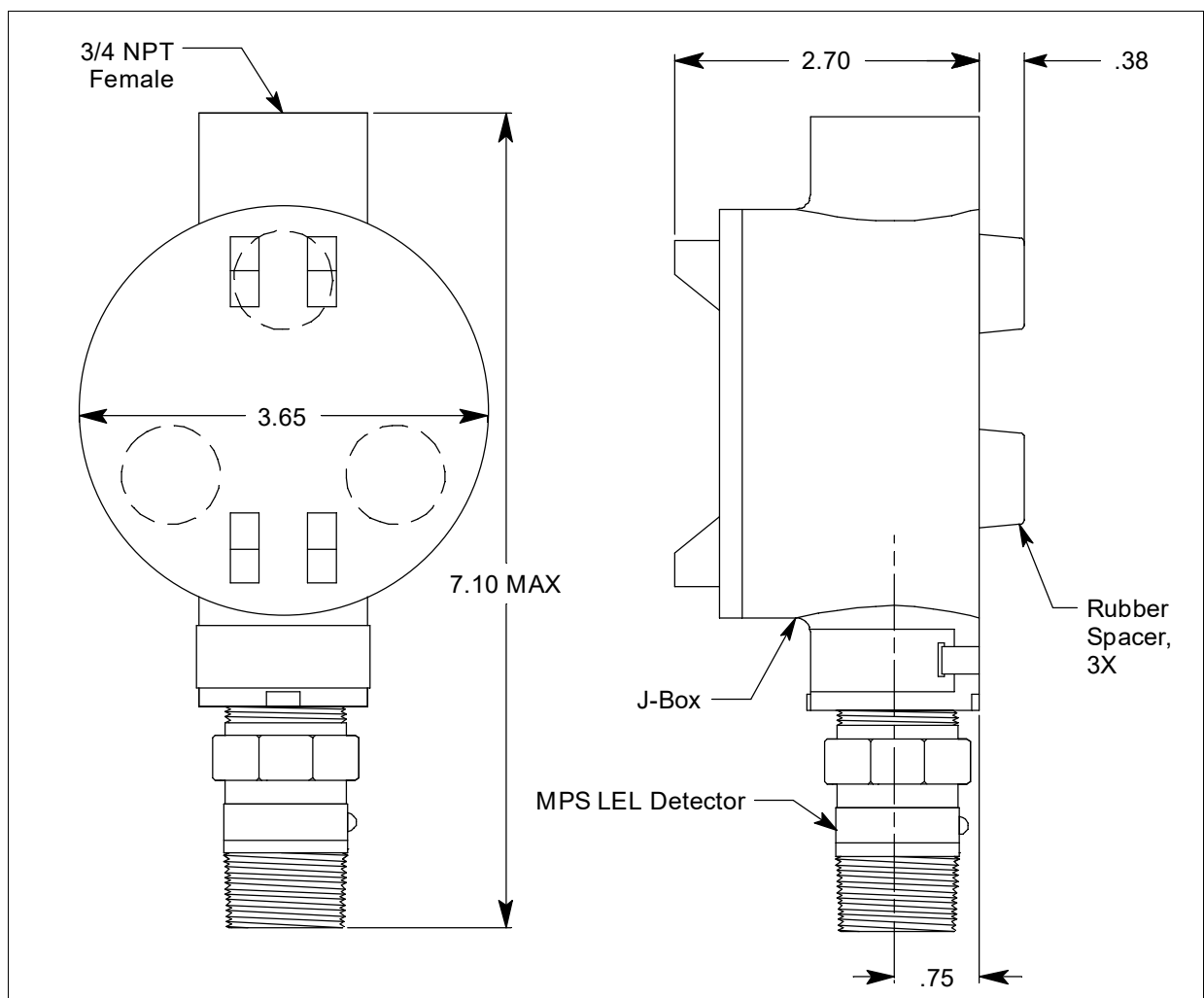
Figure 3: Mounting the Combustible Gas Transmitter
