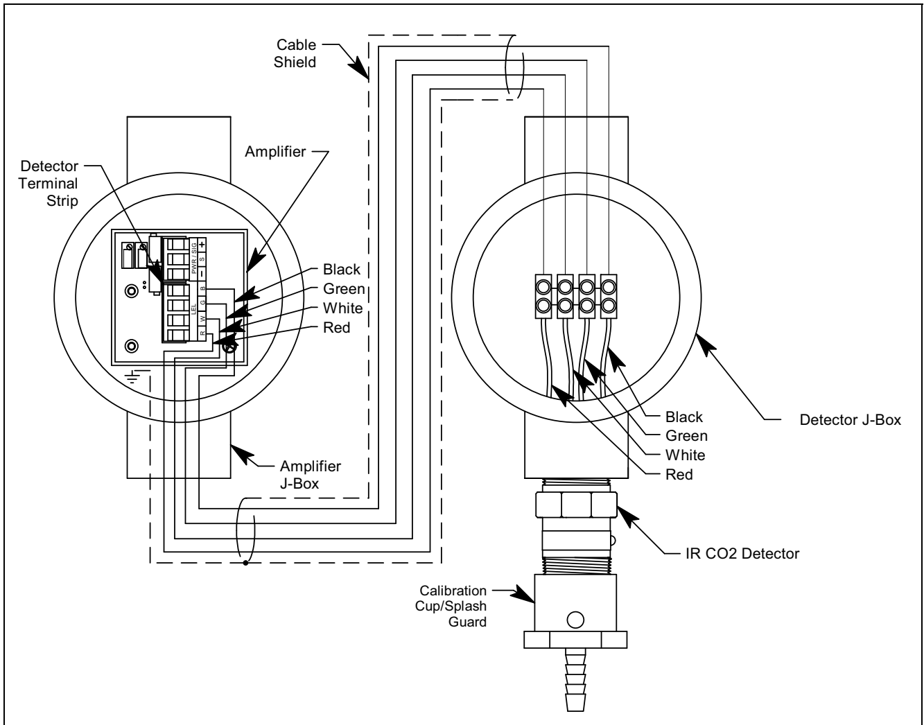
Figure 4: Wiring the Detector to the Amplifier
