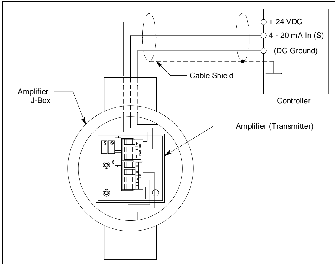
Figure 5: Wiring the Amplifier to a Controller
