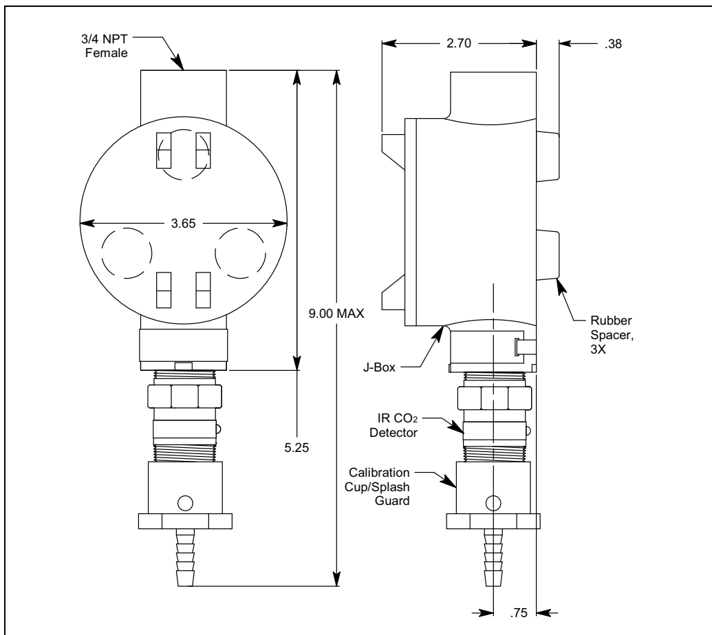
Figure 3: Mounting the CO 2 Transmitter
