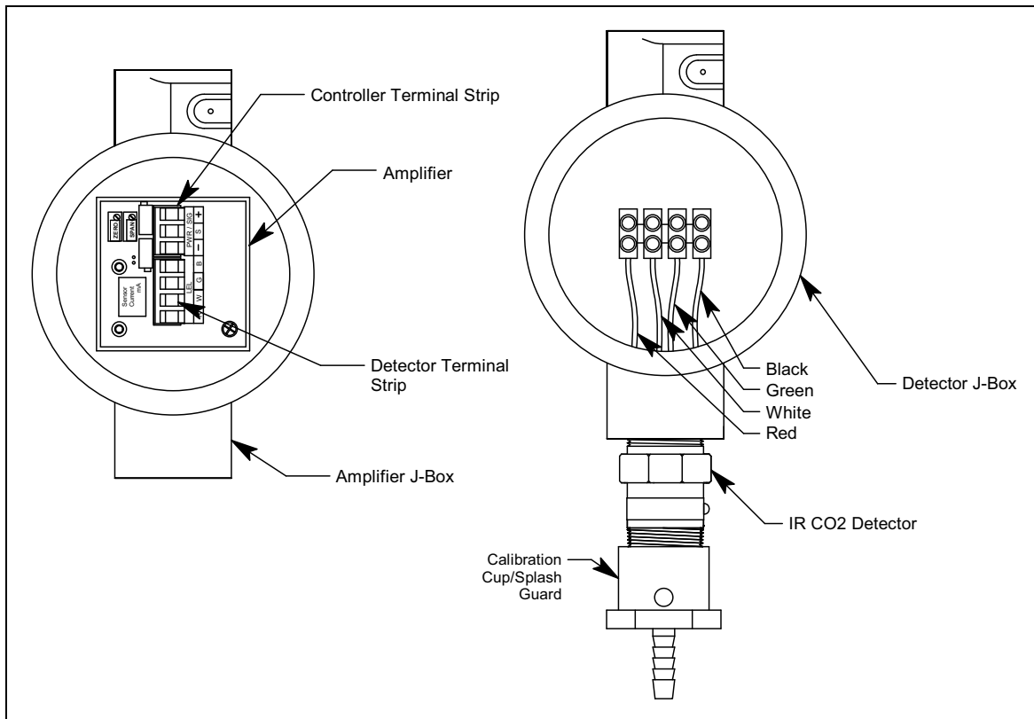
Figure 1: CO 2 Transmitter Component Location
