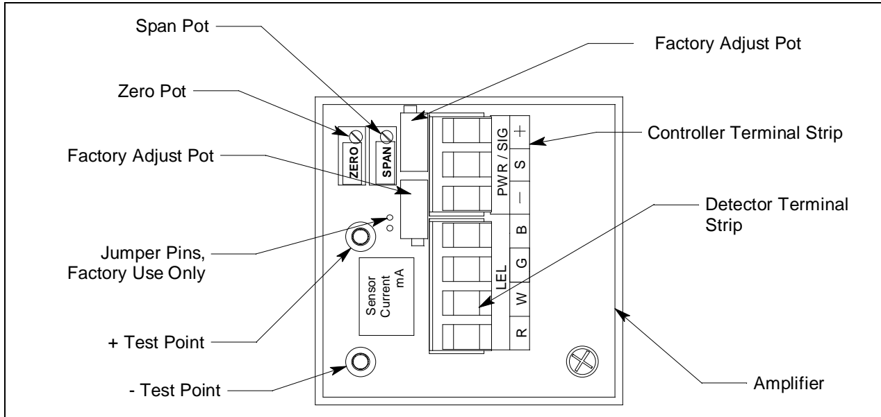
Figure 2: Amplifier Component Location
