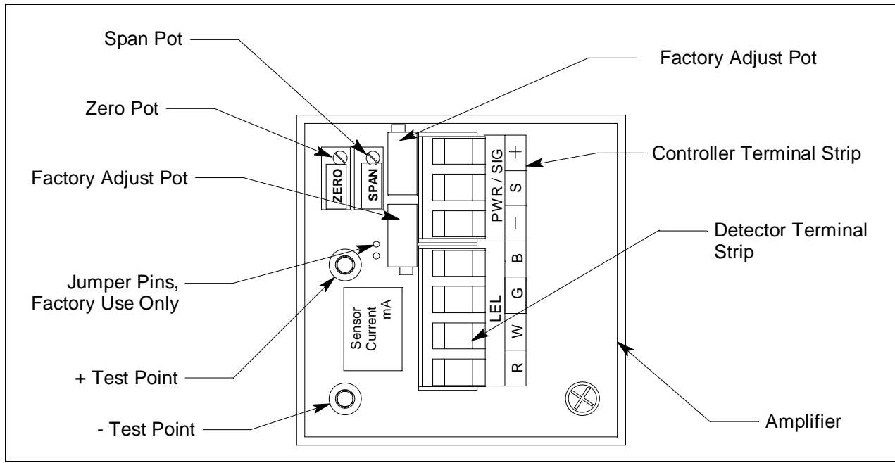
Figure 3: Amplifier Component Location
