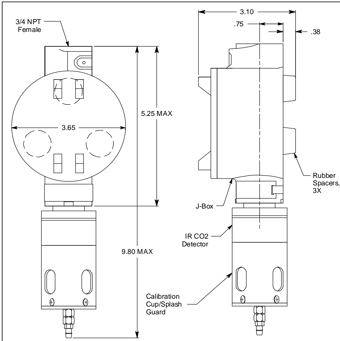
Figure 4: Mounting the CO 2 Transmitter
