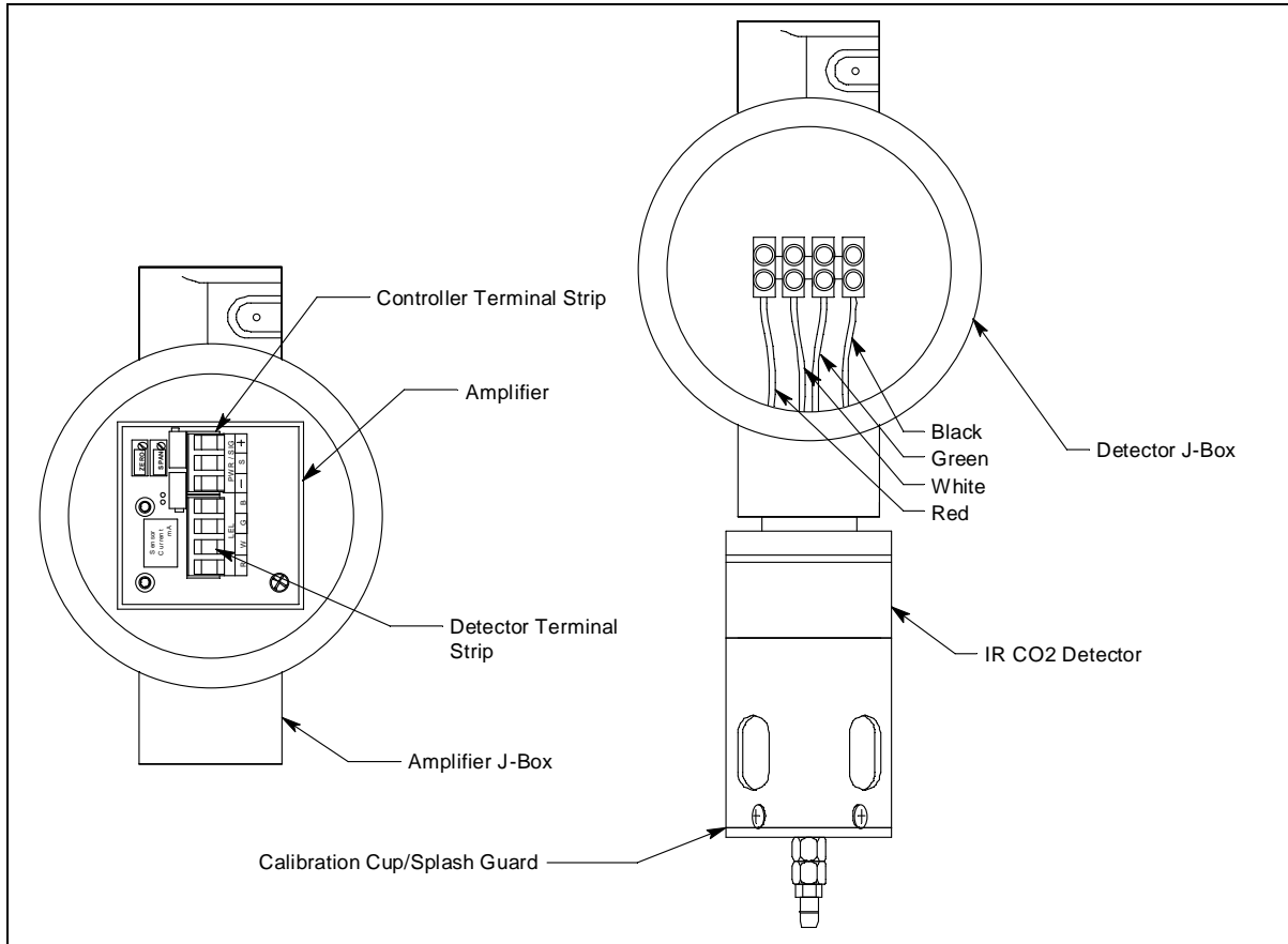
Figure 1: CO 2 Transmitter Component Location
