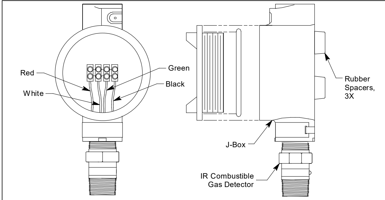
Figure 1: Component Location
