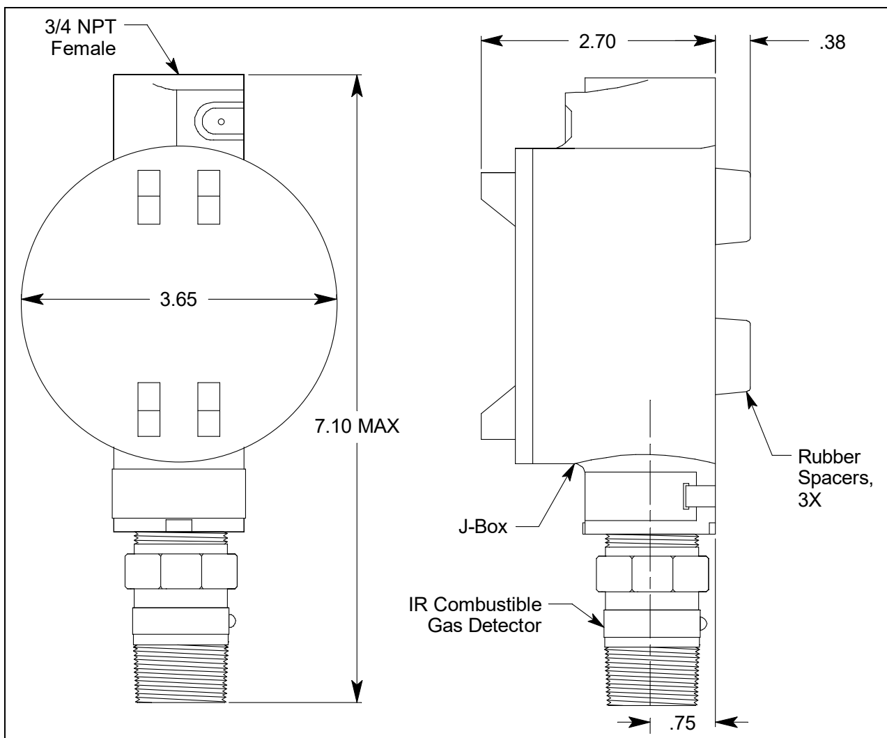
Figure 2: Mounting the Combustible Gas Detector
