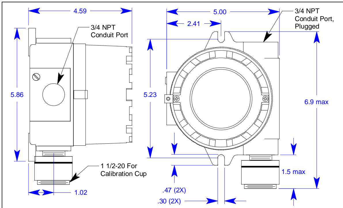
Figure 19: Outline & Mounting Dimensions, Replaceable Sensor, H 2 S, CO, and Oxygen, Non-Explosion Proof
