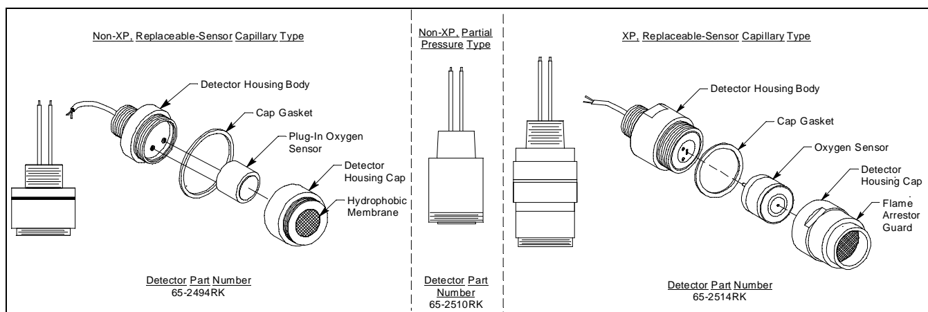
Figure 5: Oxygen Detectors
