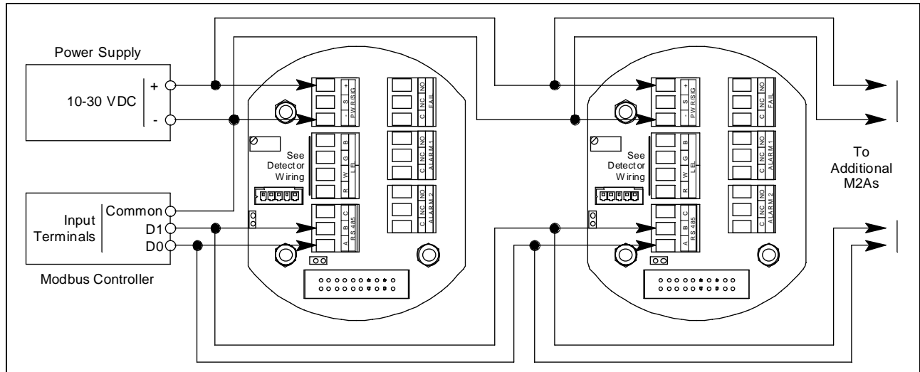
Figure 36: Alternate Modbus Wiring
