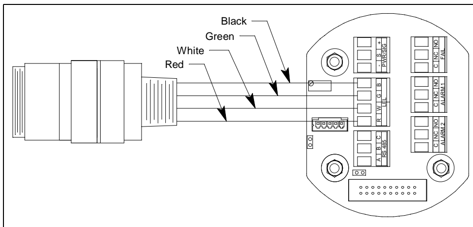
Figure 25: Replaceable IR LEL and IR CO 2 Detector Wiring
