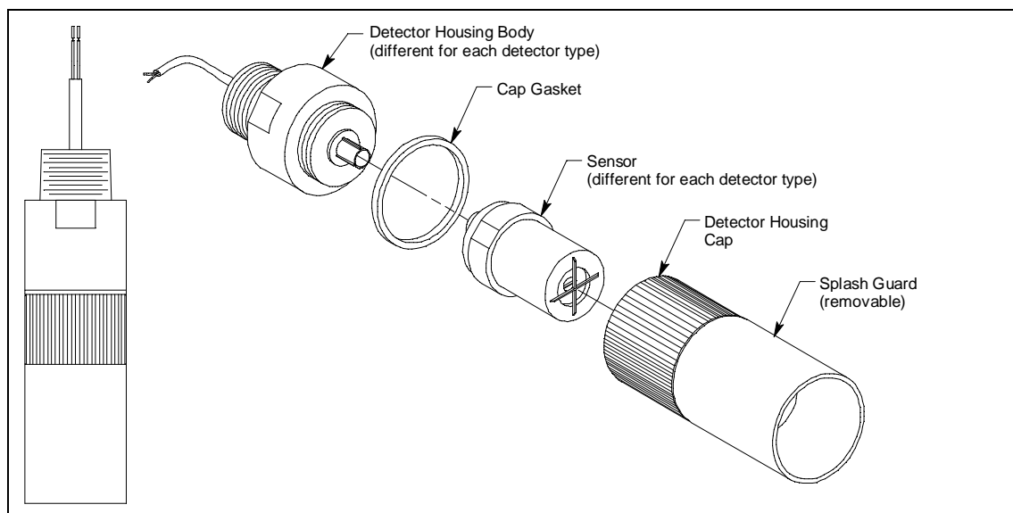
Figure 8: ESM-01 Type Detector
