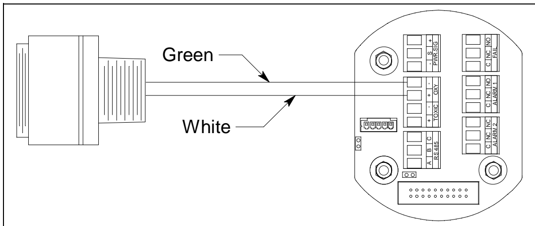
Figure 28: Capillary Type Replaceable Sensor Oxygen Detector Wiring
