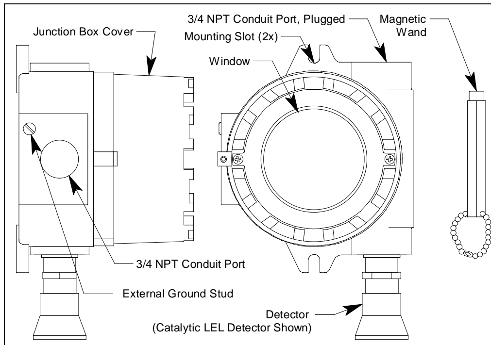
Figure 1: M2A External Components
