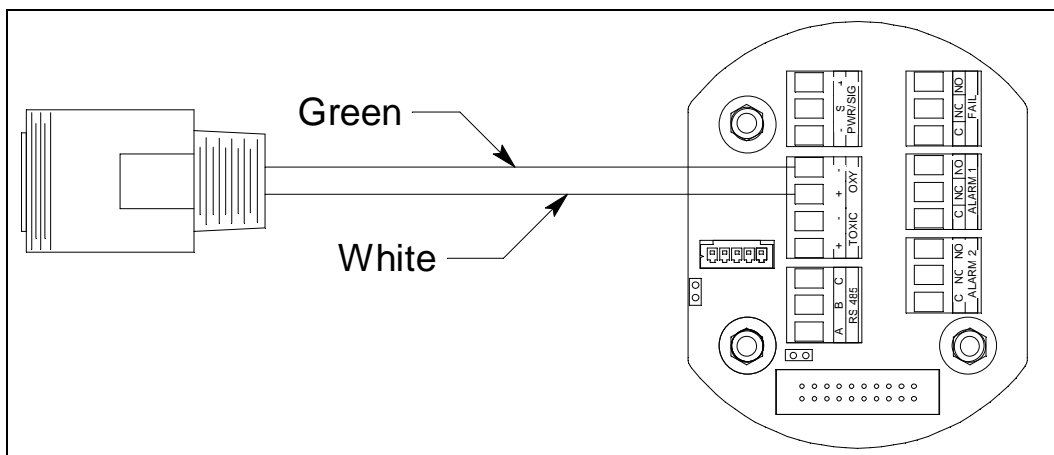
Figure 26: Partial Pressure Oxygen Detector Wiring
