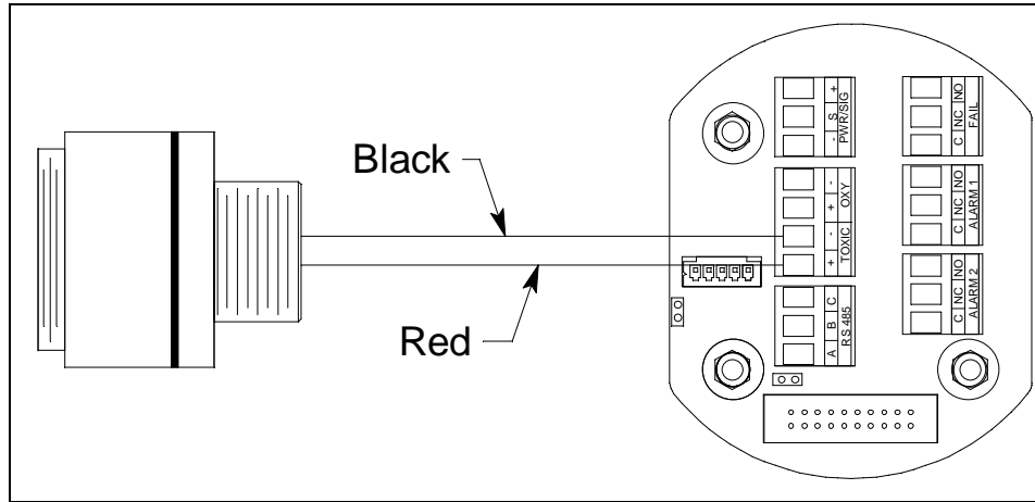
Figure 30: H 2 S/CO Detector Wiring
