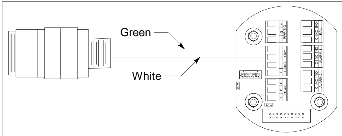
Figure 27: CSA Capillary Type Oxygen Detector Wiring
