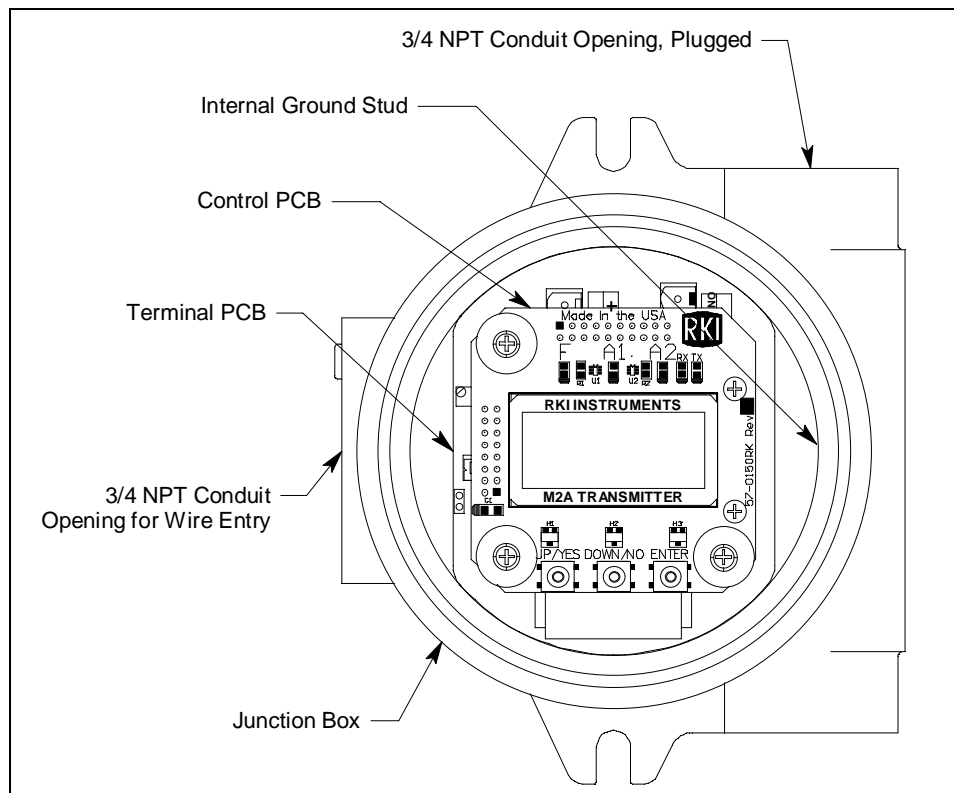
Figure 11: M2A Internal Components
