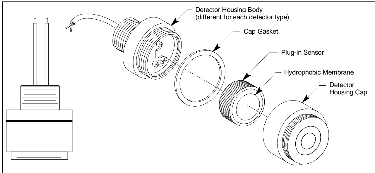
Figure 9: CT-7 Series Detectors
