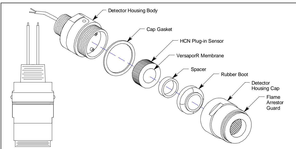
Figure 10: Explosion-Proof CT-7 Series HCN Detector
