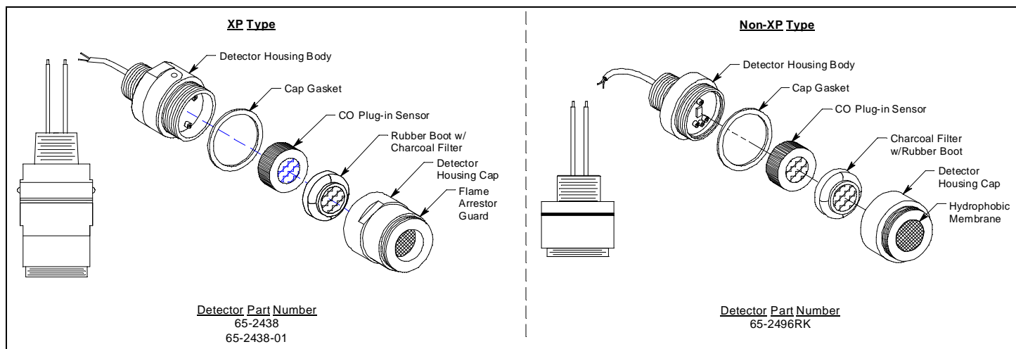
Figure 7: CO Detectors
