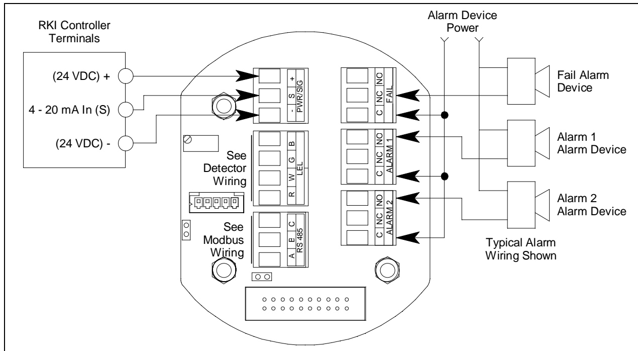
Figure 33: Wiring the M2A to a Controller and Alarm Devices
