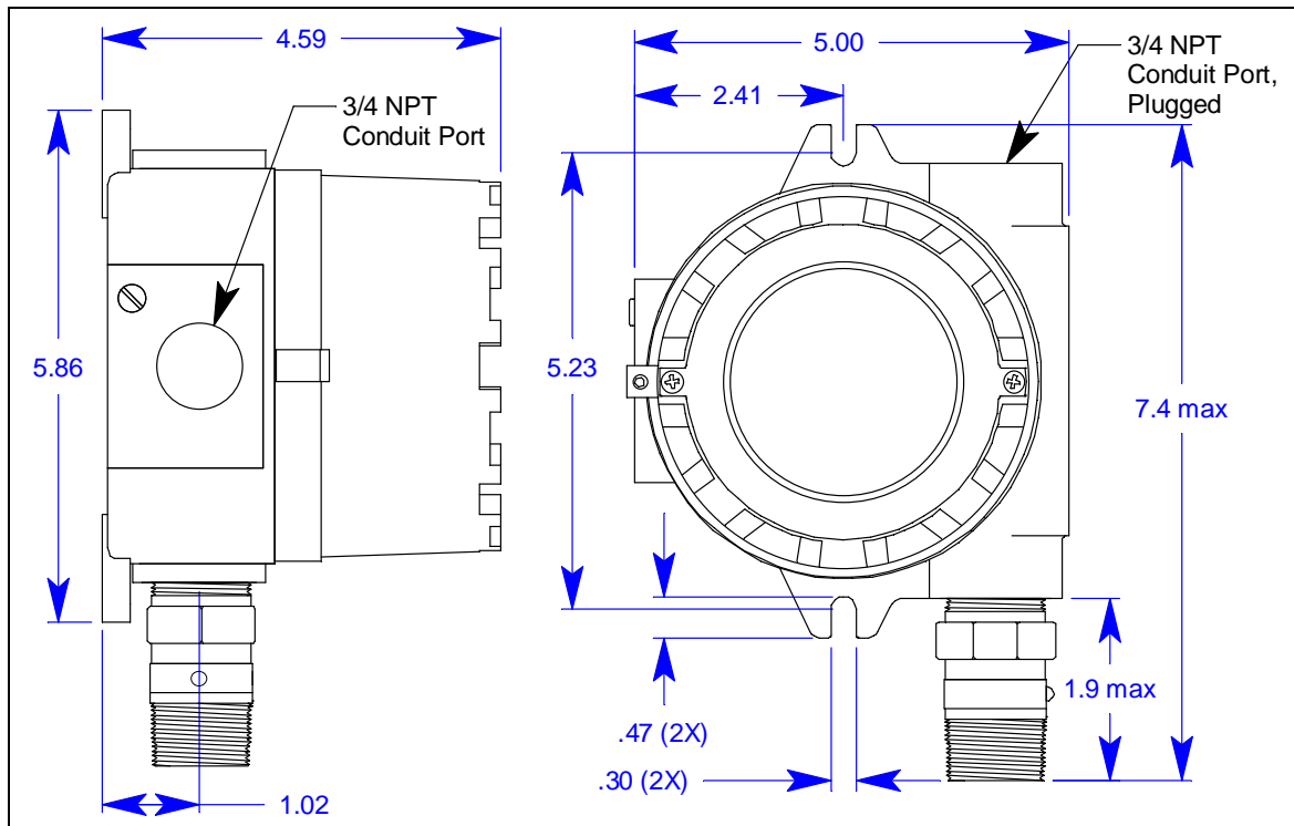
Figure 17: Outline & Mounting Dimensions, IR Combustible, CO 2 , and MPS LEL Detectors
