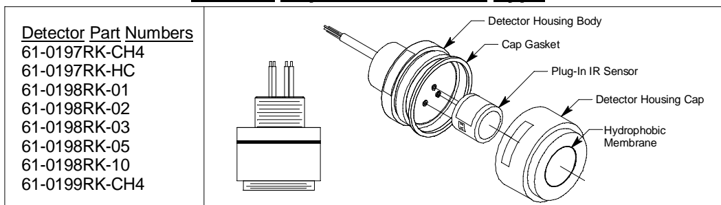
Figure 4: Non-XP Infrared (IR) Detectors
