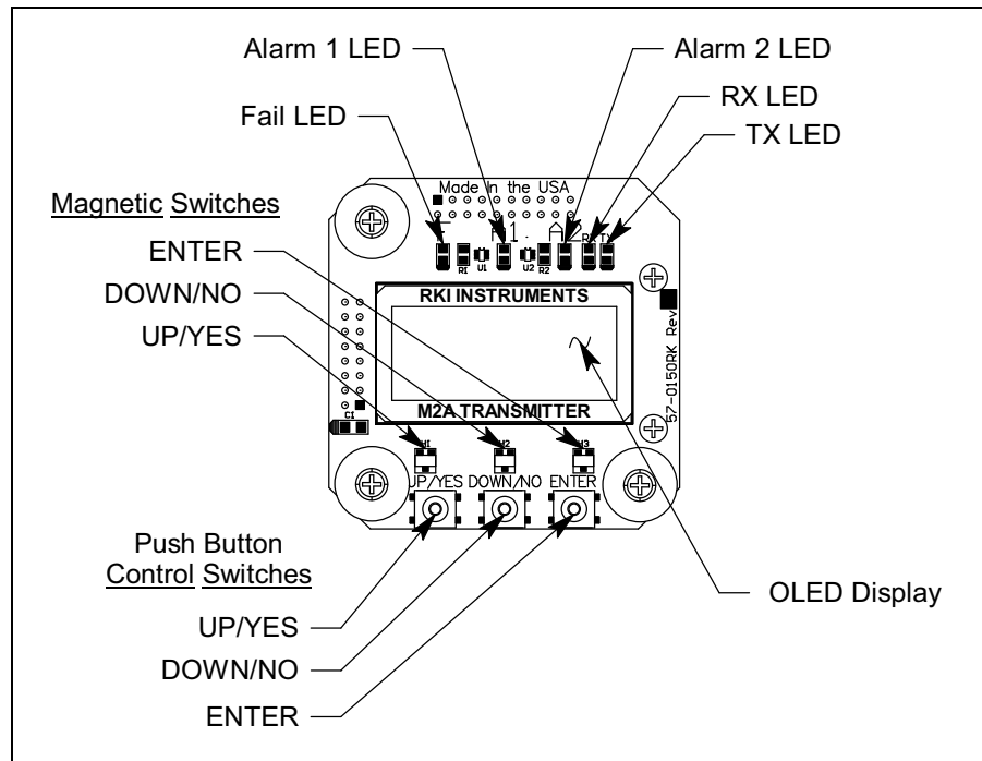
Figure 14: Control PCB Component Location
