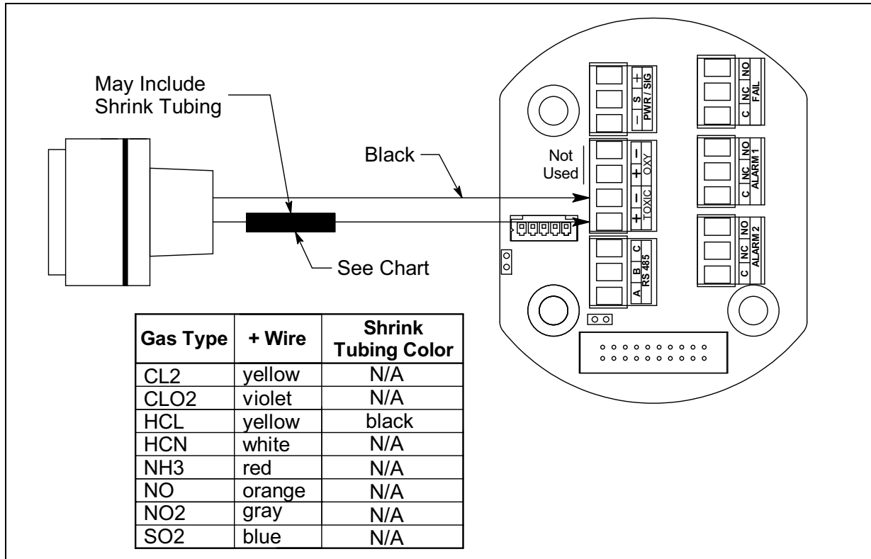
Figure 32: Non-Explosion Proof CT-7 Series Toxic Detector Wiring
