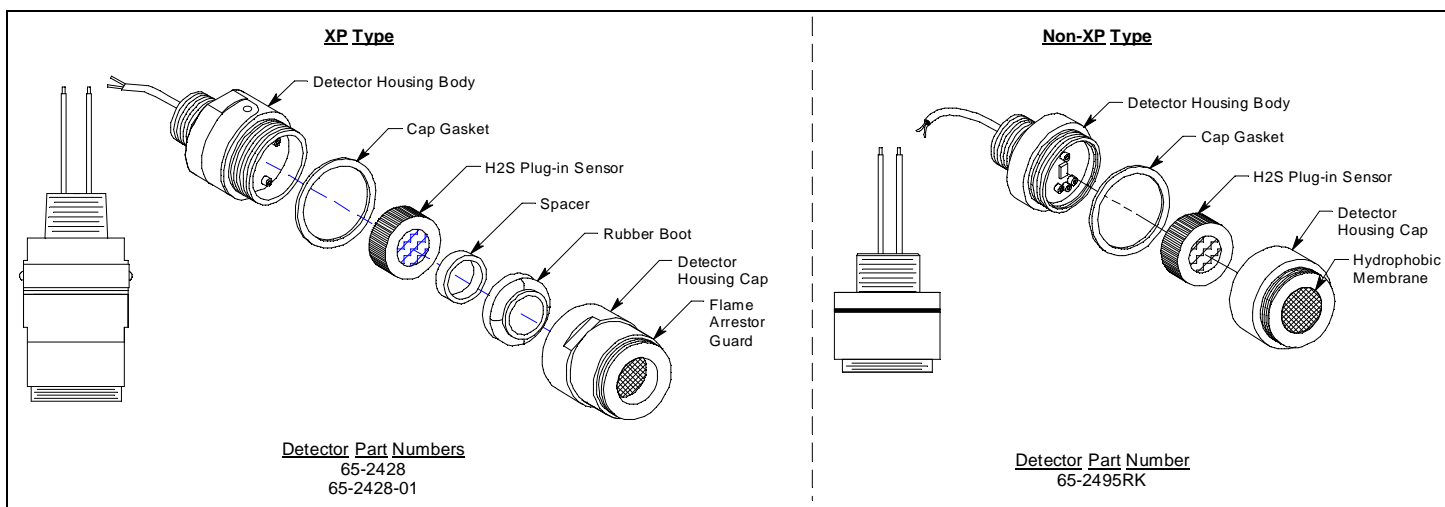
Figure 6: H 2 S Detectors
