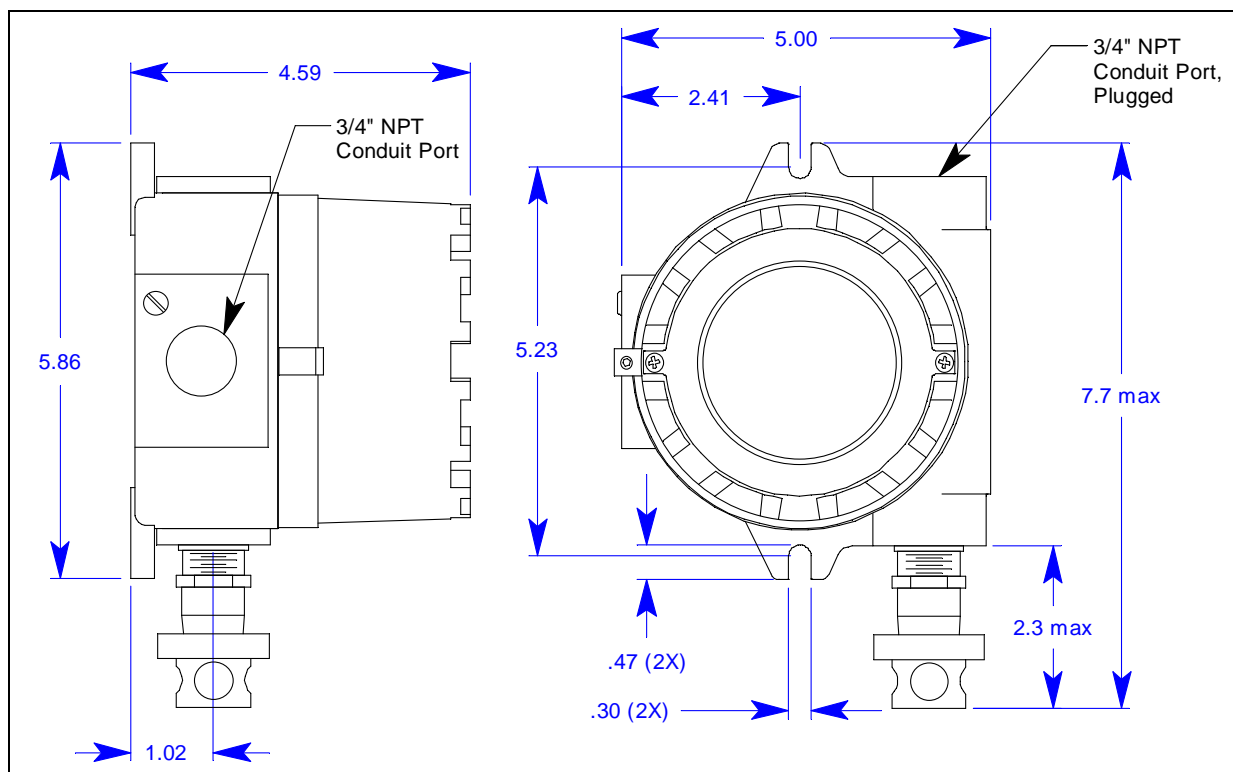
Figure 16: Outline & Mounting Dimensions, Catalytic LEL and ppm, CSA Version
