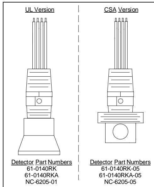
Figure 2: Catalytic Detectors
