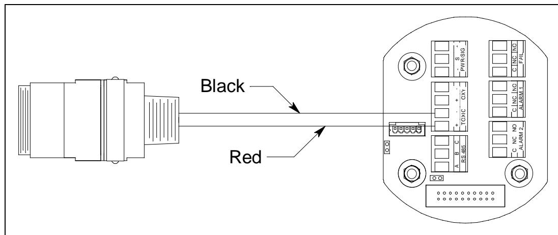
Figure 29: H 2 S/CO/HCN Detector Wiring, CSA
