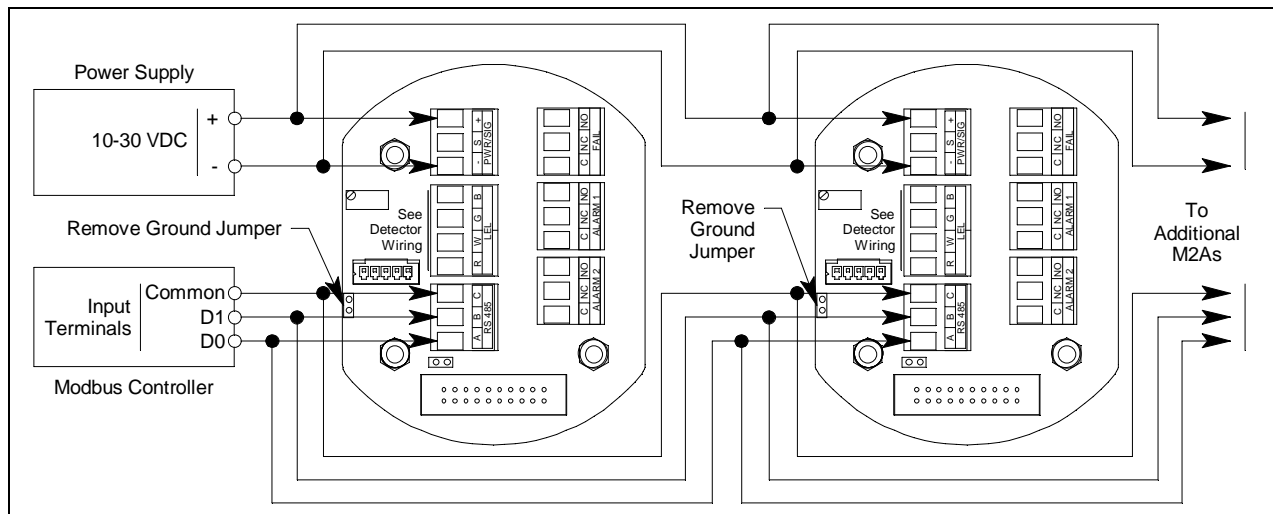
Figure 35: Recommended Modbus Wiring
