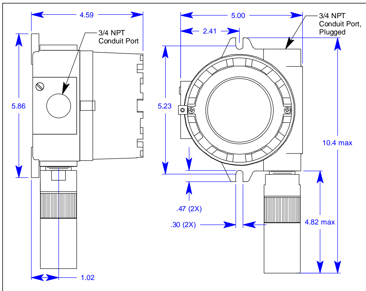
Figure 21: Outline & Mounting Dimensions, ESM-01 Toxic
