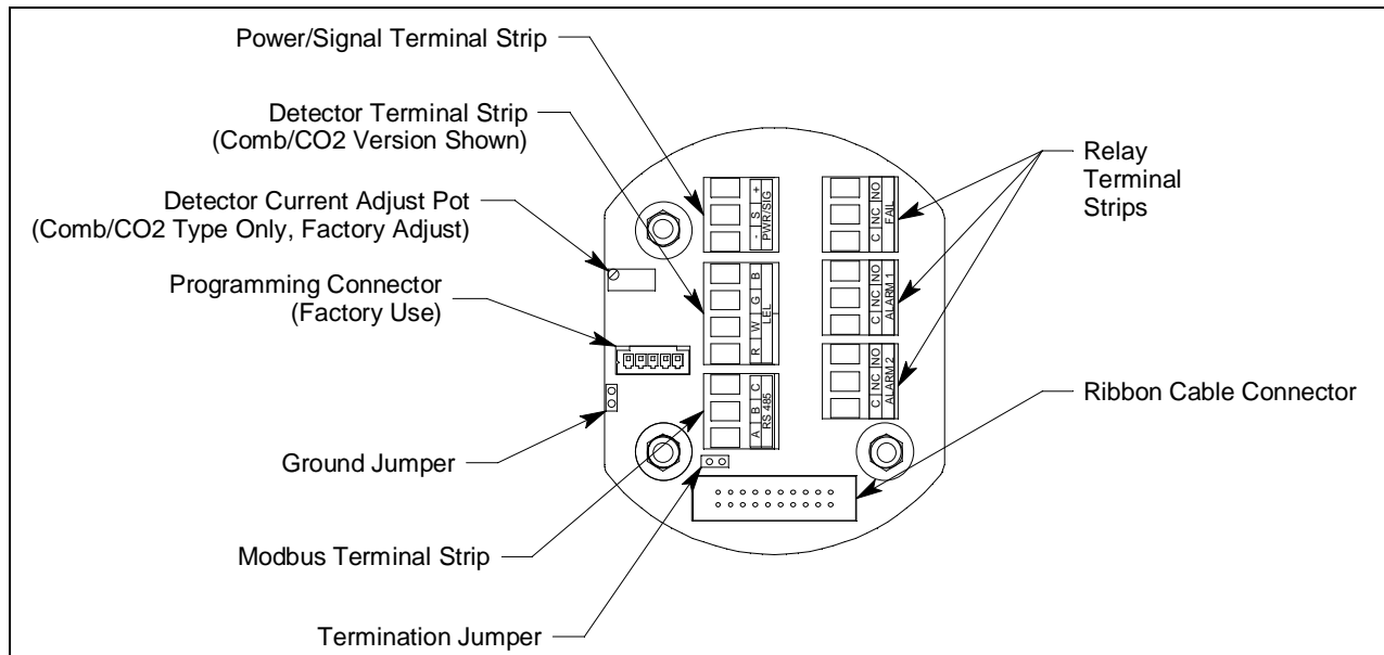
Figure 12: Terminal PCB Component Location
