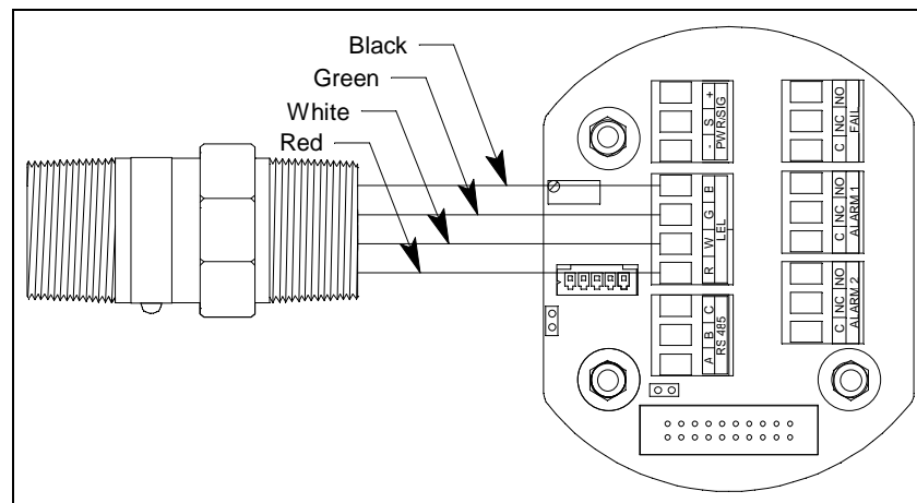
Figure 24: IR Combustible and IR CO 2 /MPS LEL Detector Wiring
