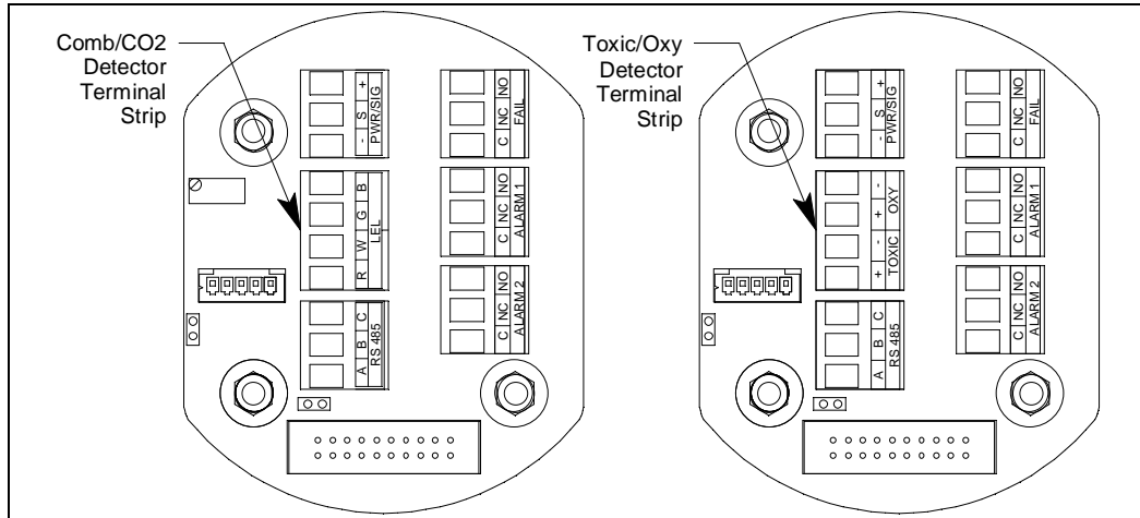
Figure 13: Detector Terminal Strip
