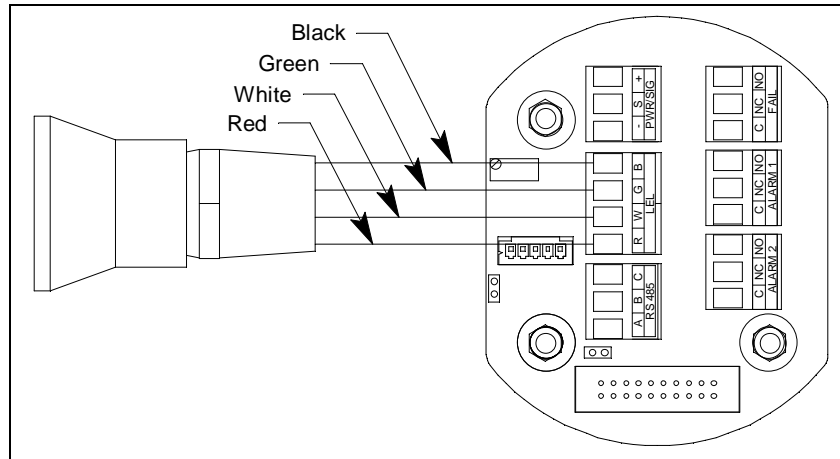
Figure 23: Catalytic LEL and ppm Detector Wiring
