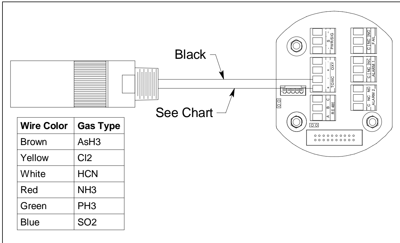
Figure 31: ESM-01 Toxic Detector Wiring
