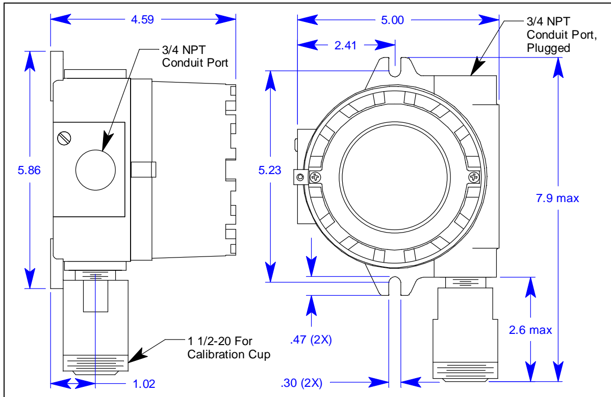
Figure 18: Outline & Mounting Dimensions, Oxygen, Partial Pressure Type
