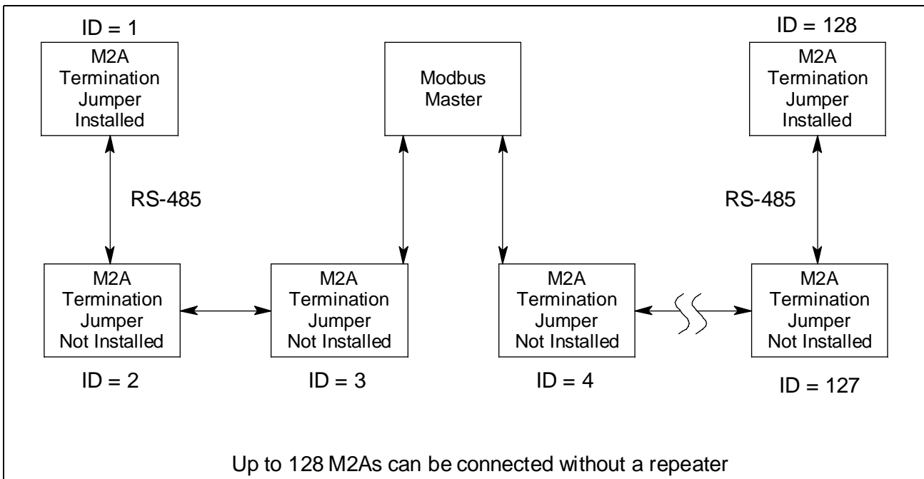
Figure 38: Multiple M2As in a Two Branch Configuration
