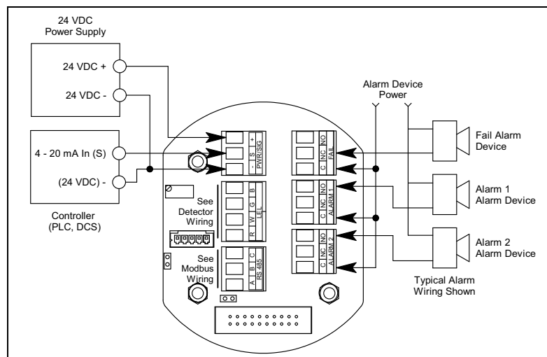
Figure 39: PLC and DCS Device Wiring
