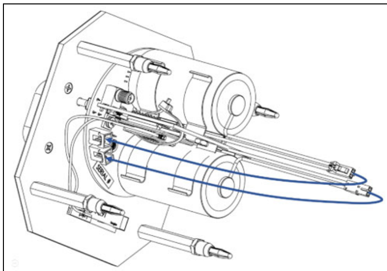
Figure 6: Battery Connection
