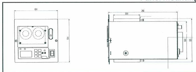
Panel mounting
