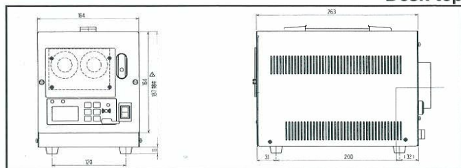
Desk top
