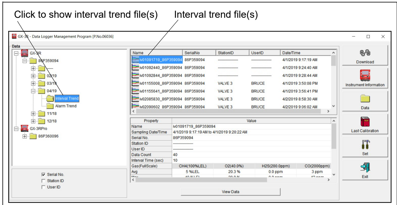
Figure 21: Data Window - Selecting Interval Trend Files
