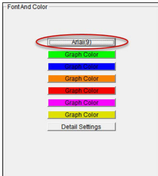
Figure 52: Font Button
