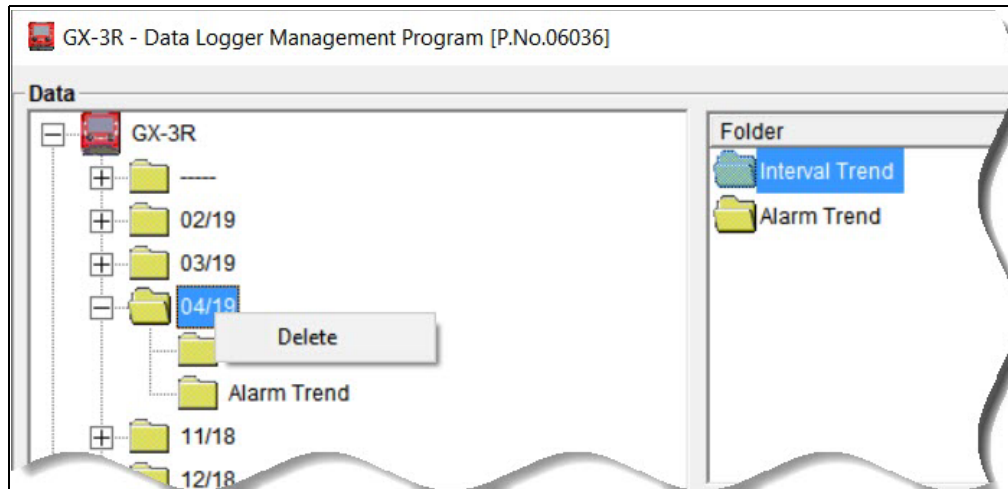
Figure 30: Delete Box
