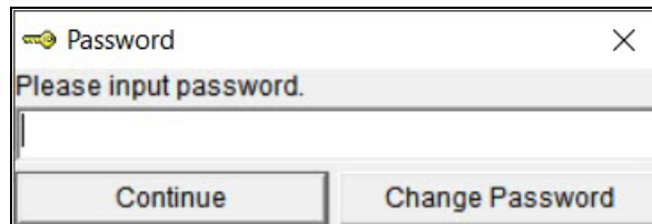
Figure 29: Password Window
