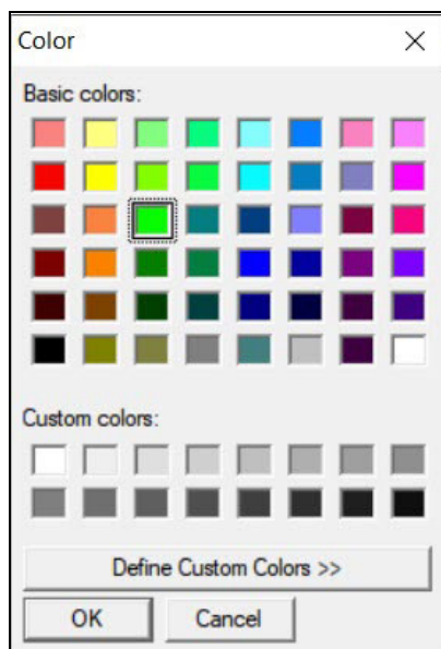
Figure 55: Color Windows
