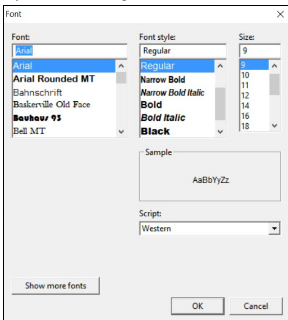
Figure 53: Font Window
