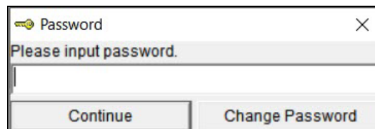
Figure 42: Password Window
