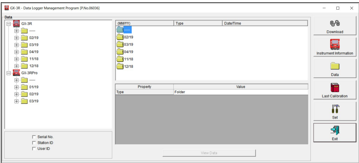
Figure 13: Data Window
