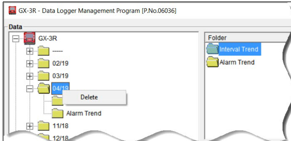
Figure 28: Delete Box
