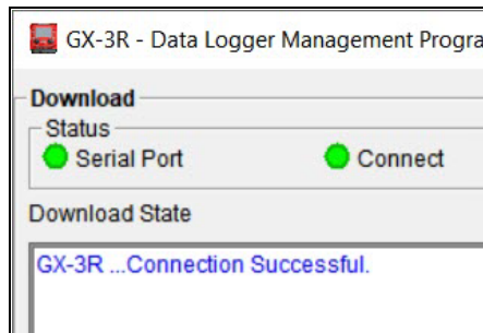
Figure 7: Connection Message
