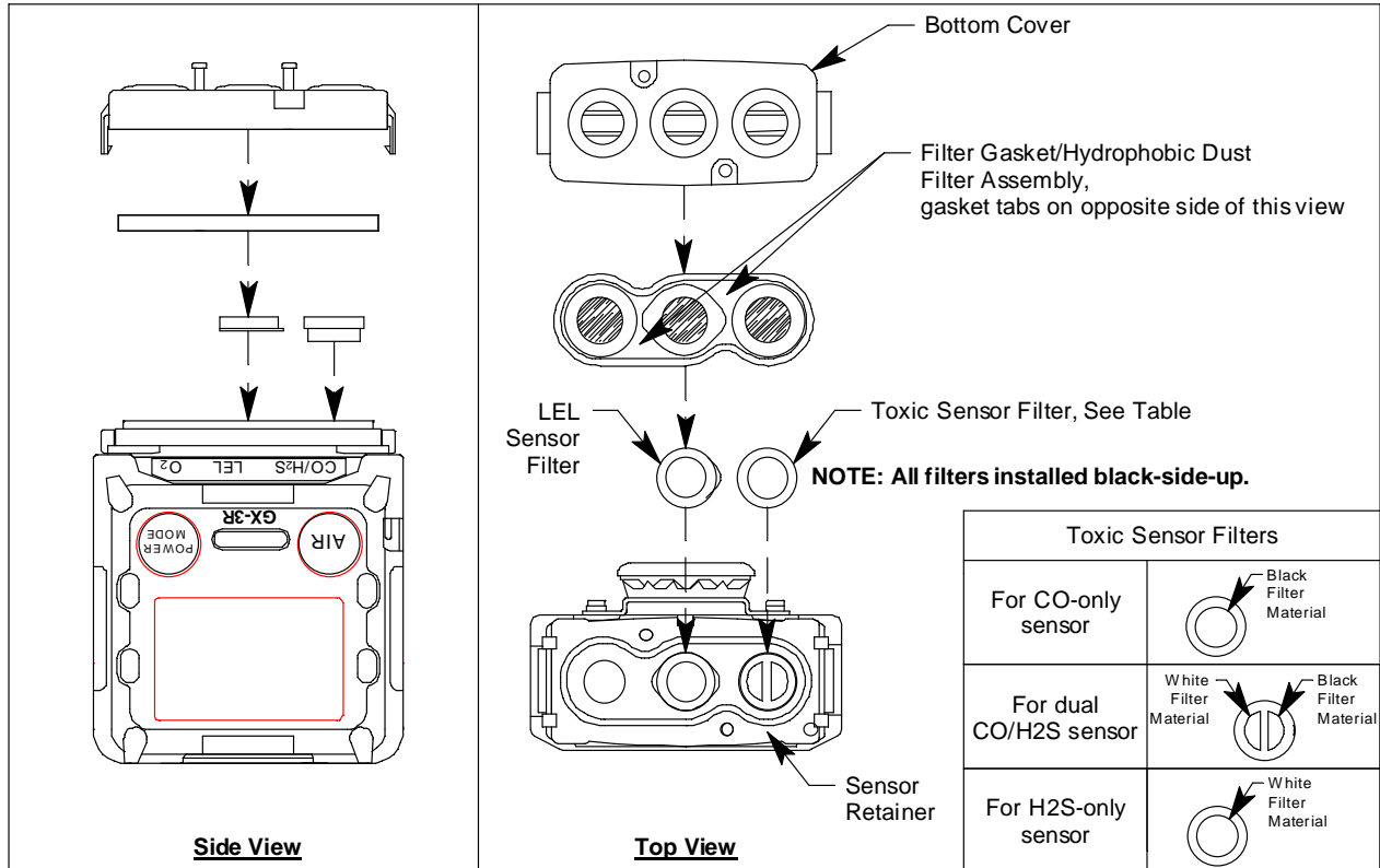
Figure 14: Replacing the Sensor Filters
