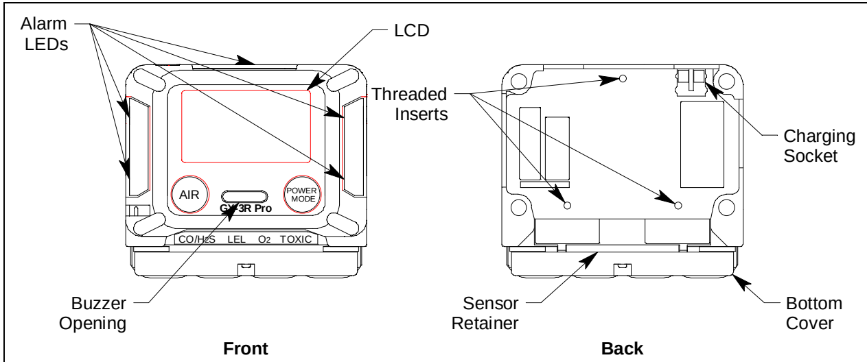
Figure 1: Component Location
