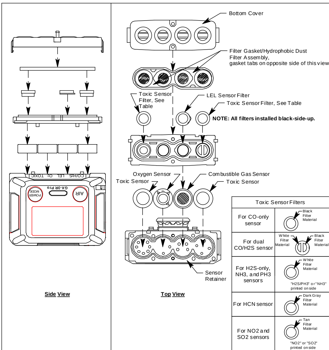
Figure 18: Replacing a Sensor
