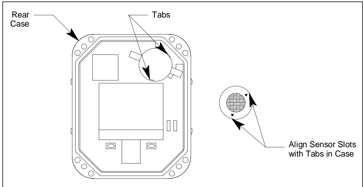
Figure 16: Sensor Location
