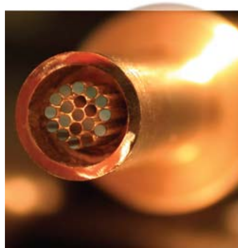
Free-standing bundle of 19 fibers, 600 \mu m core
