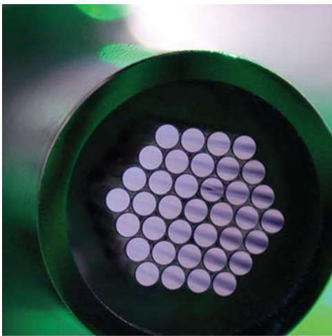
Free-standing, tightly packed hexagonal bundle of 37 fibers, 600 \mu m core
